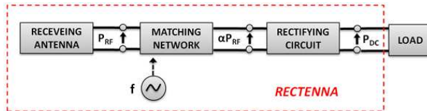
Figure 1. Energy harvesting architecture.
